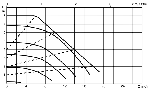
EVOPLUS B 80/220.40 M - EVOPLUS D 80/220.40 M
