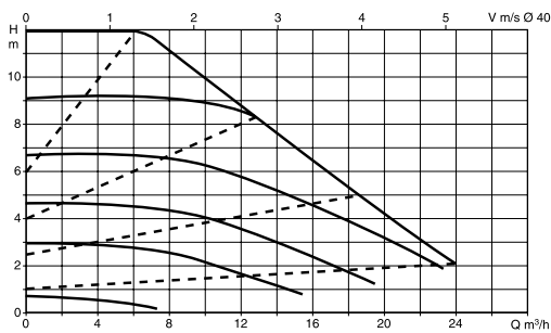
EVOPLUS B 120/250.40 M - EVOPLUS D 120/250.40 M
