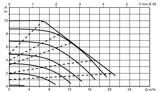
EVOPLUS B 100/220.40 M - EVOPLUS D 100/220.40 M
